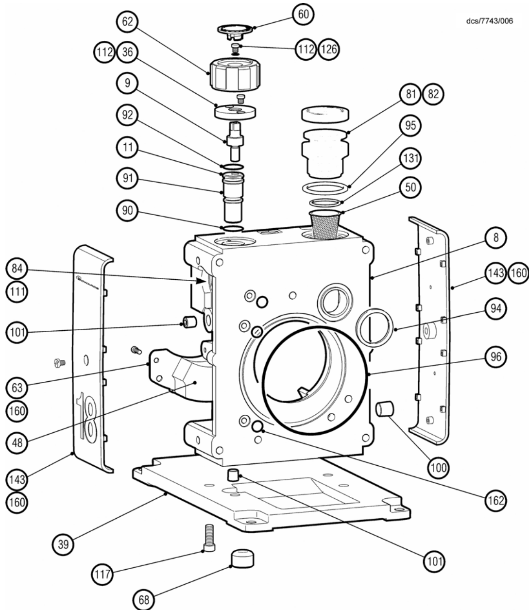
Figure 1 - Adaptor sub-assembly
