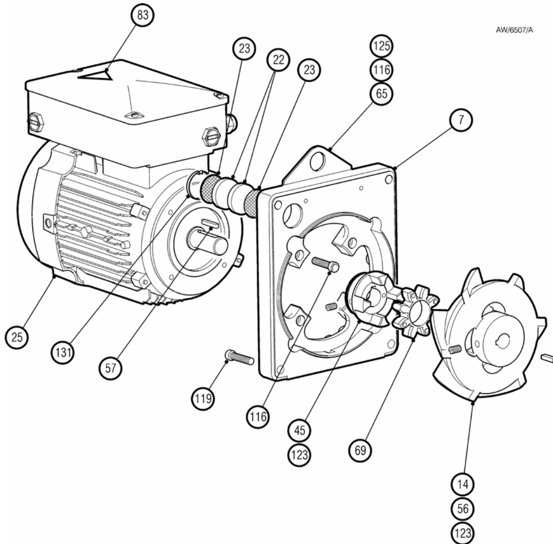
Figure 5 - Motor and adaptor plate sub-assembly
