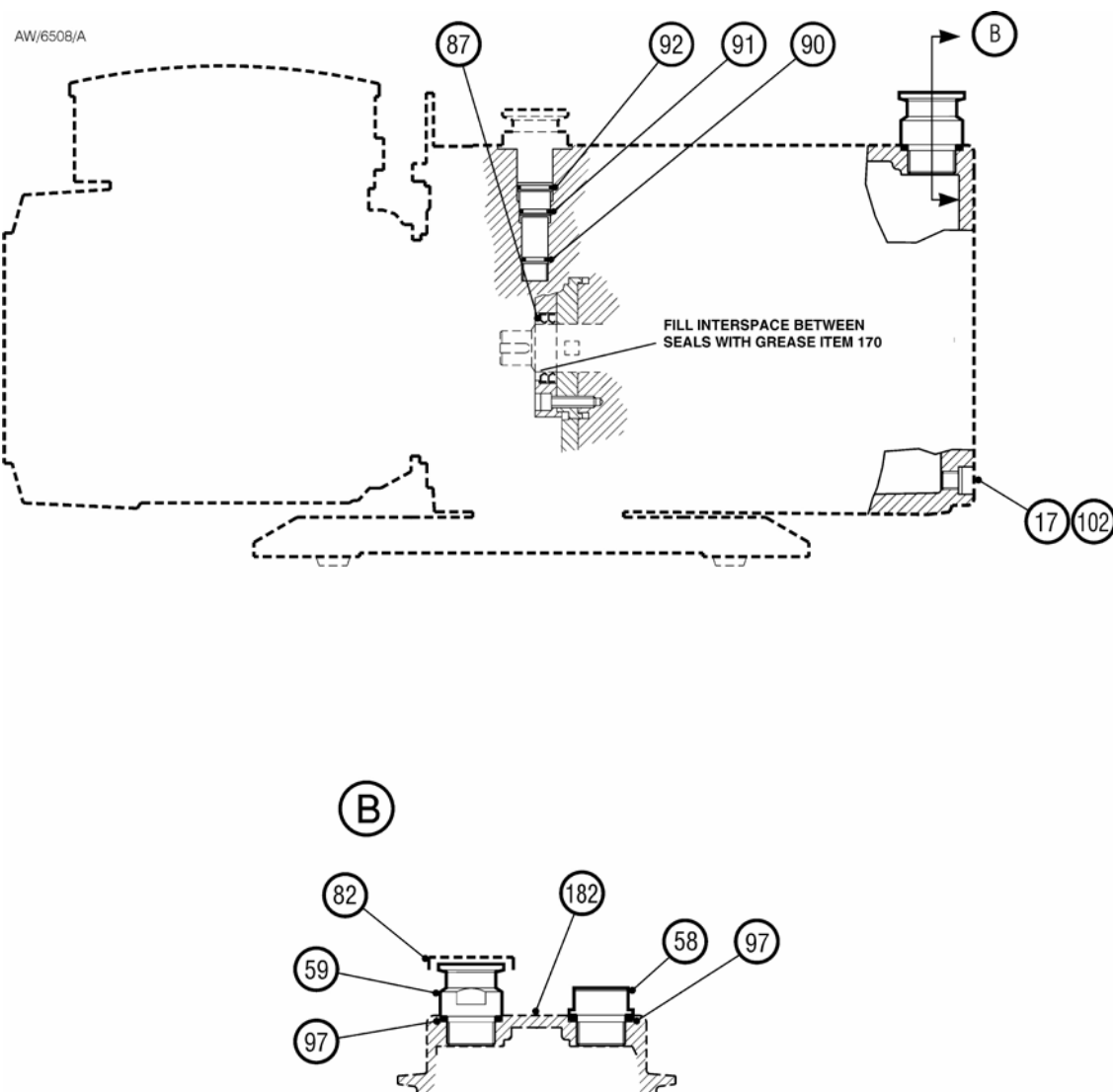
Figure 6 - Fomblin filled pumps
