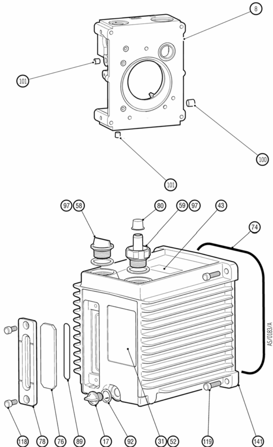
Figure 9 - E2M18 O-ring sealed oil box conversion kit
