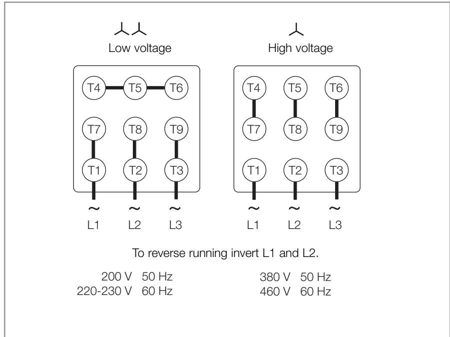
Fig. 8.3 Motor connection diagram (motor P/N: 72260067)
