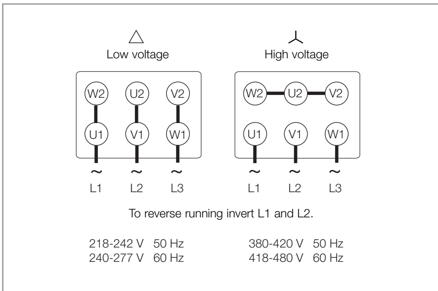
Fig. 8.2 Motor connection diagram (motor P/N: 38066006)
