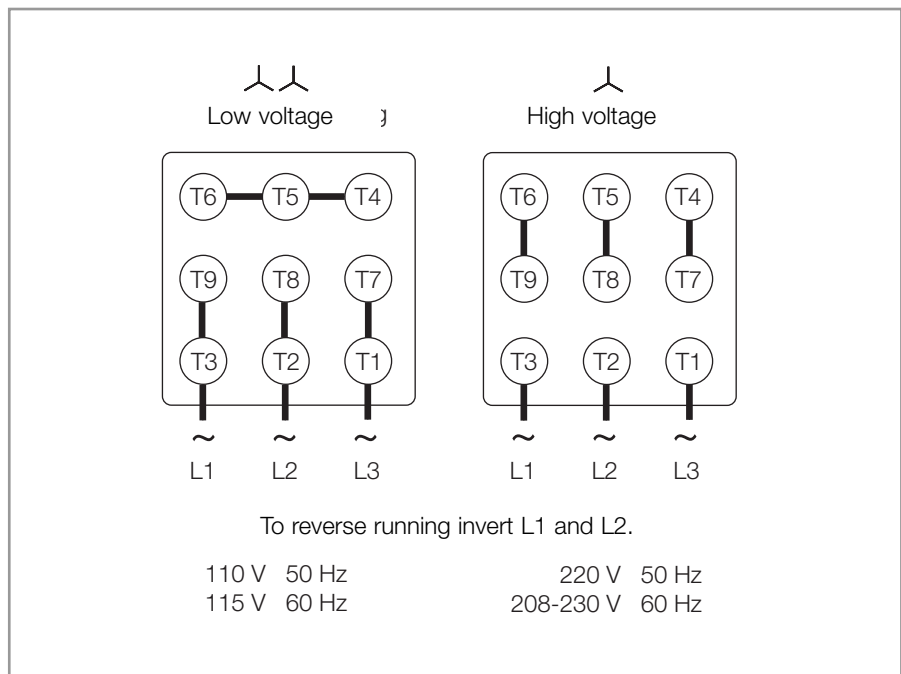
Fig. 8.4 Motor connection diagram (motor P/N: 72260135)
